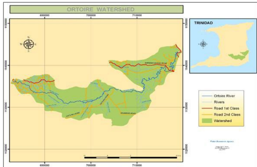
Figure 1: Map of Ortoire Watershed
