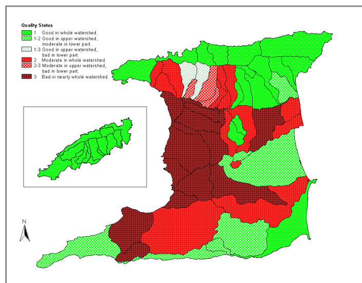
Figure 2: map showing Water Quality Status in T&T
