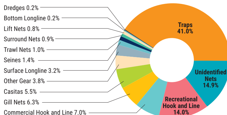
Figure 3.1.3 Type and Relative Contribution of Fishing Gear Reported as ALDFG in the Caribbean
