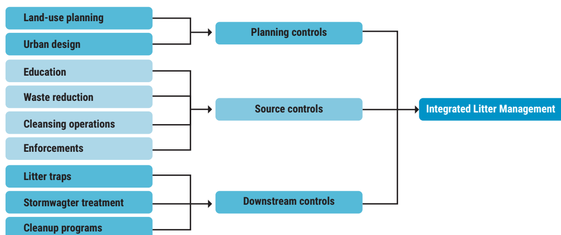
Figure A4.2 Solving the Problem—Integrated Litter Management Strategy
