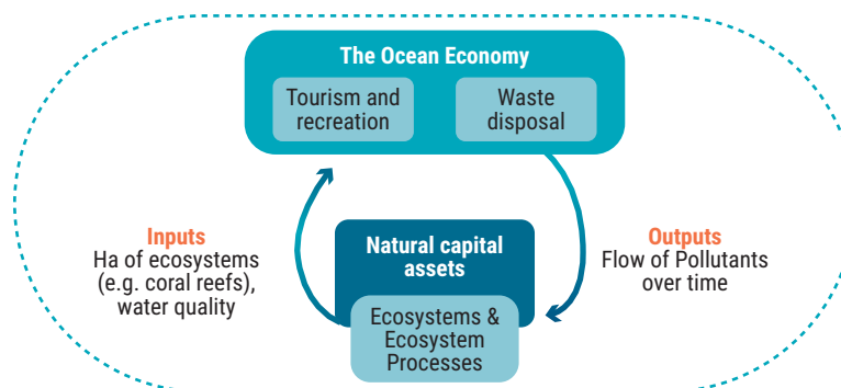
Figure 1.1.3 Blue Economy Linkages: Tourism, Waste Disposal, and Ecosystems
