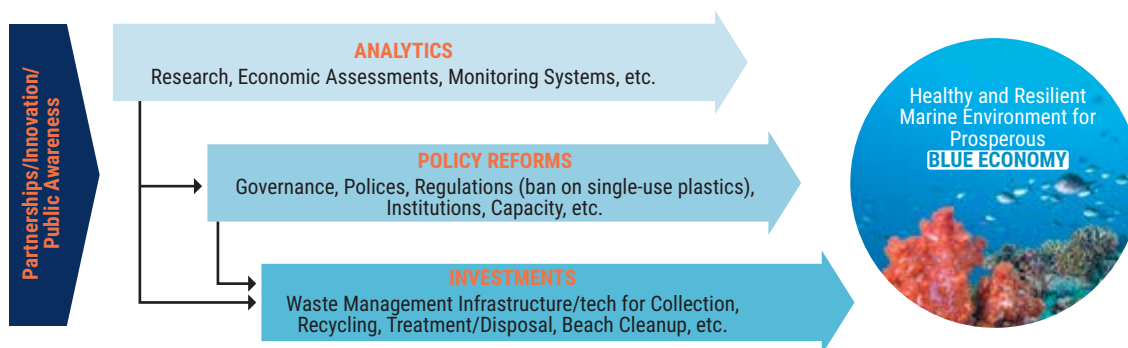
Figure 5.1.1 Framework for Action to Address Marine Pollution
