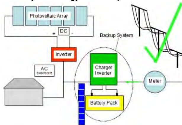
Figure 5.16: Grid connected with backup, public power supply on (GrenSol, 2012)
