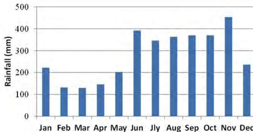
Figure 3.3b: Average monthly rainfall at Grand Etang
